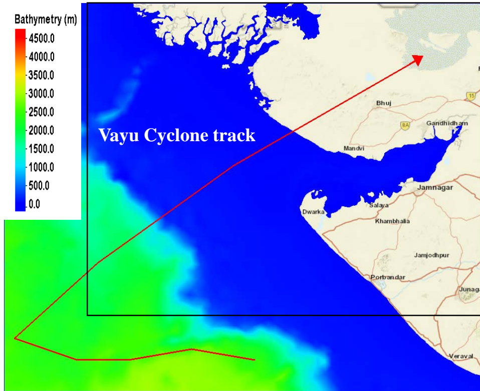
Bathymetry along with the cyclone track
