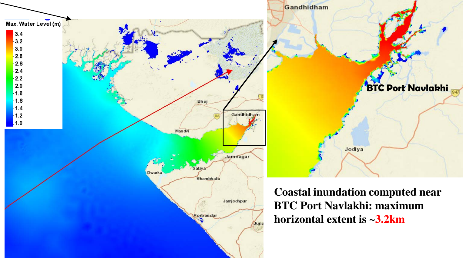
Spatial distribution of maximum storm surge including tide and inundation for the box region
